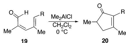
SCHEME 8. Iso-Nazarov Cyclization to Give Cyclopentenones
