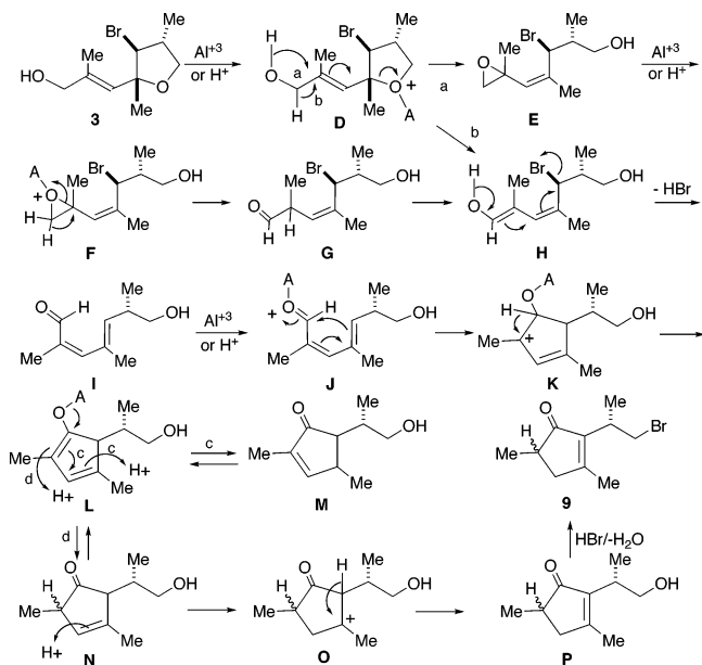
SCHEME 7. Proposed Mechanism for Formation of Rearrangement Product 9
